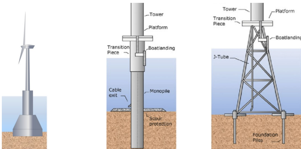
Figur 3.4 Eksempler af fundamentstyper (set fra venstre side): gravitationsfundamenter; monopæl; Jacket-type fundamenter (kilde: https://www.obayashi.co.jp/chronicle/130th/en/archives/chapter4_1_5.html# oraz: https://www.researchgate.net/figure/Three-types-of-tur
